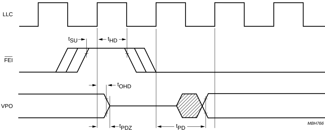
Fig.22 \overline{\text{FEI}} timing in CCIR 656 mode [OFTS (1 : 0) = 3].
