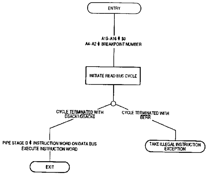
Figure 6-6. Breakpoint Instruction Flowchart
