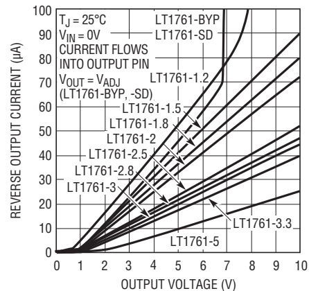
Figure 6. Reverse Output Current
