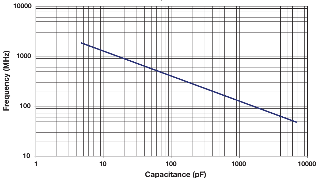
Typical Series Resonant Frequency vs. Capacitance HQ E Case
